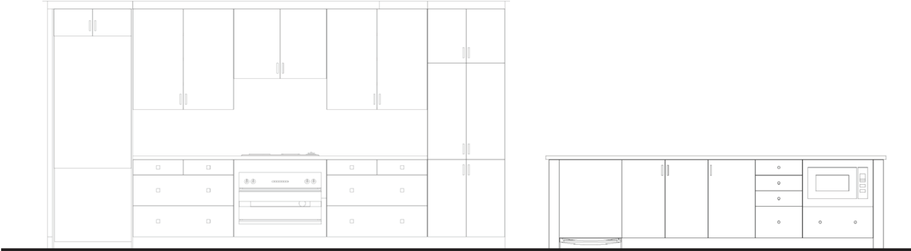
KITCHEN CABINET LAY-OUT
