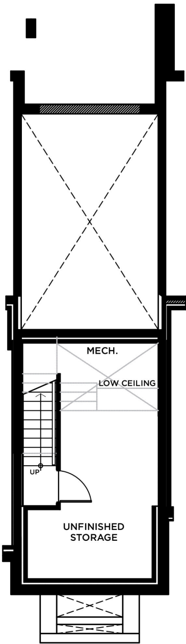
BASEMENT FLOOR PLAN
