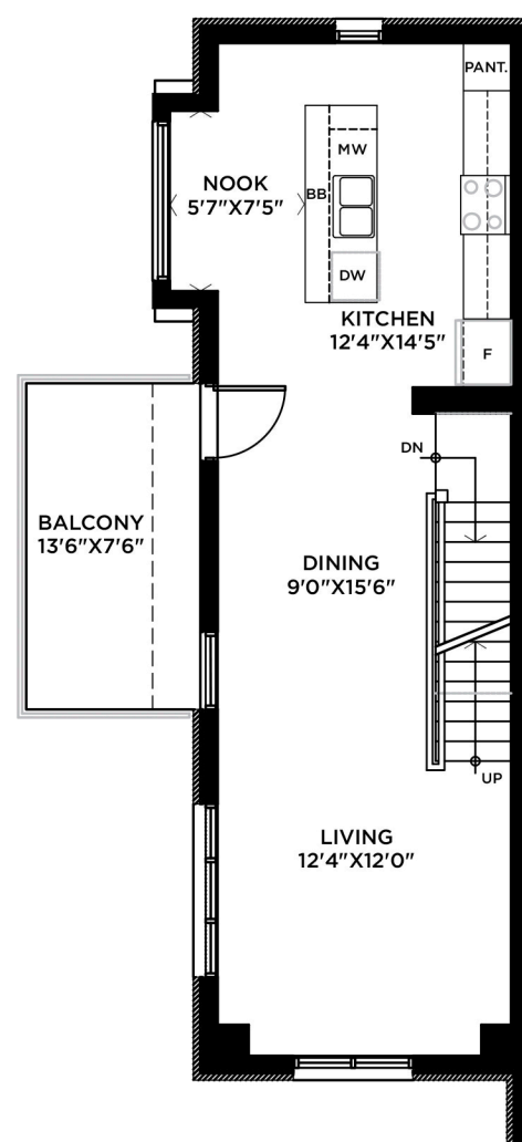
SECOND FLOOR PLAN 617 sq. ft.
